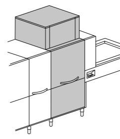
DRF99M + 900 mm 9 kW Stage dryer
